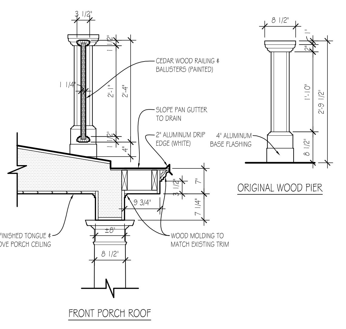
FRONT PORCH ROOF
