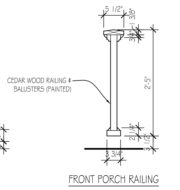
FRONT PORCH RAILING
